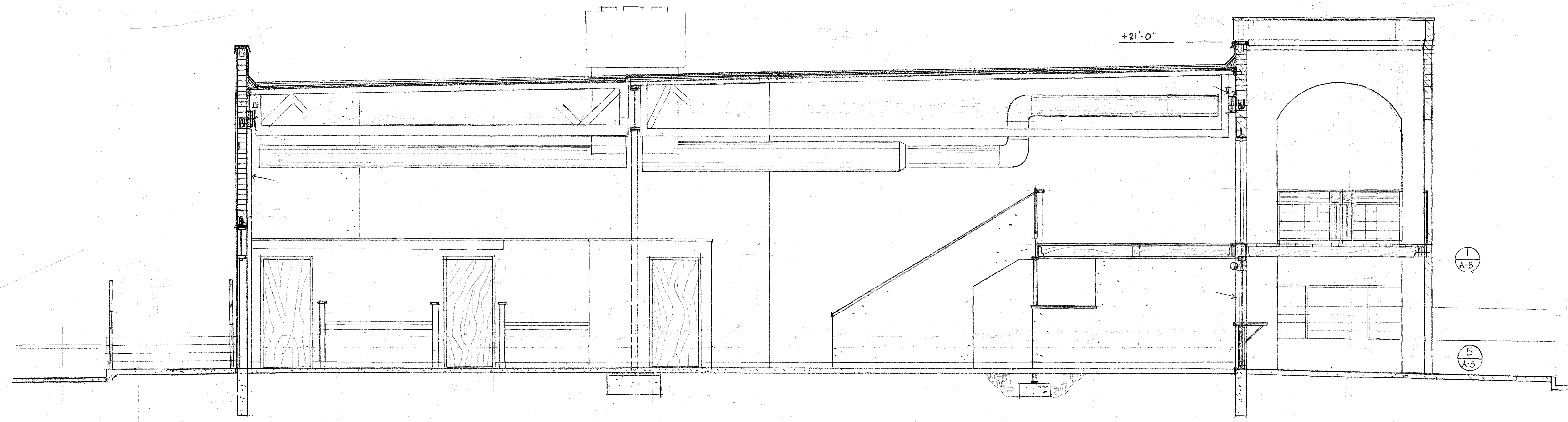
Section 1/4" = 1'-0"
