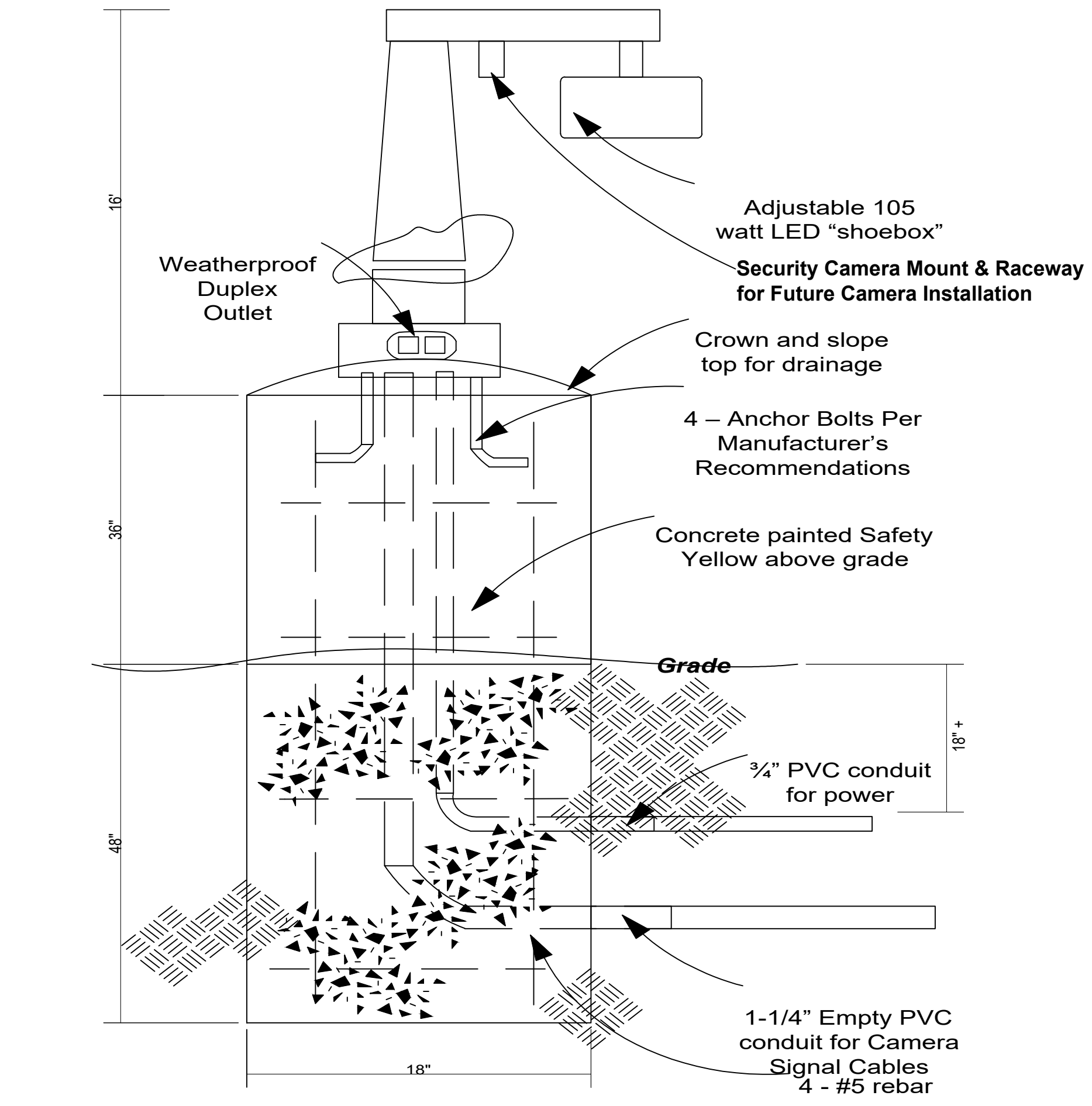
2 Parking Lot Pole Detail E3
